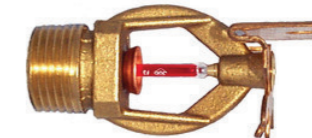
Pendent Type Sprinkler Upright Type Sprinkler Sidewall Type Sprinkler Concealed Type Sprinkler
